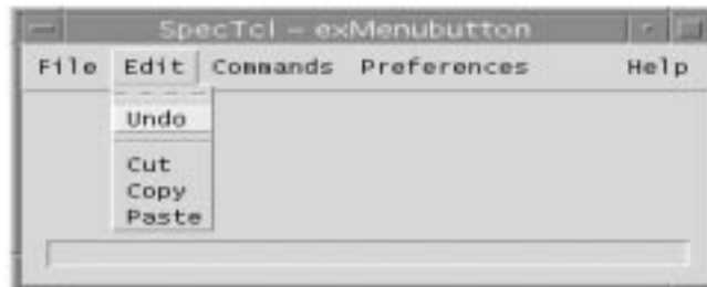
Figure 6-10 Menu Application
