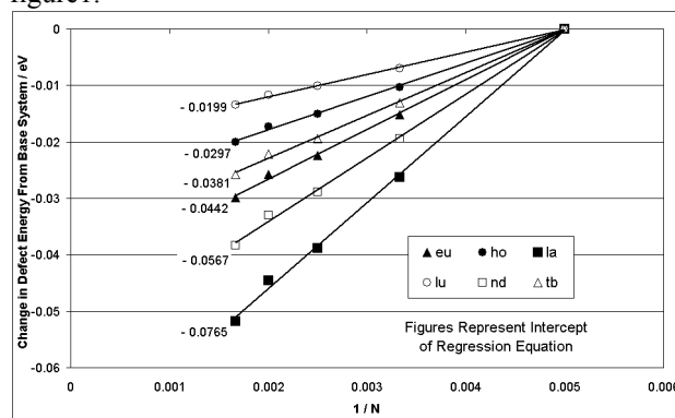
Figure 1: convergence of defect energy with system size for cations on the surfaces of goethite.
