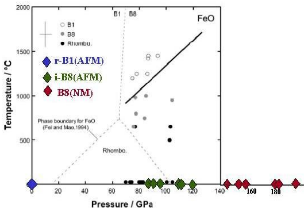
Figure 12: phase diagram of FeO showing transitions.
