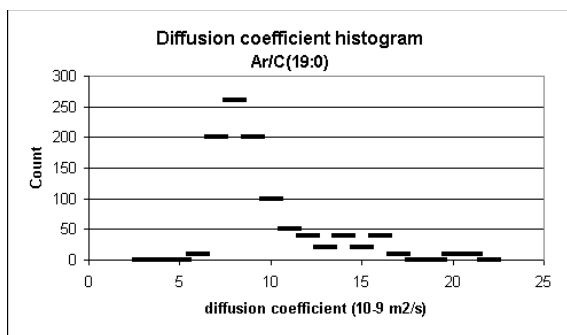
Figure 4: distribution of diffusion coefficients for Ar in a carbon nanotube.
