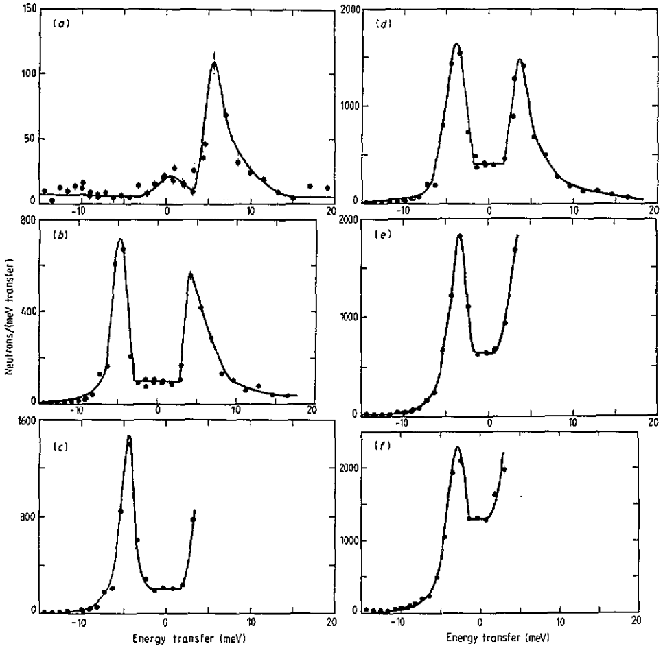
Figure 7. The spectra shown at (a) 10 K, (b) 293 K, (c) 373 K, (d) 473 K, (e) 573 K, and (f) 773 K are constant- Q extractions from the set of time of flight spectra.
