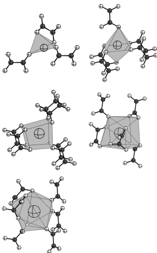
Figure 7. Coordination polyhedra of crystal structures of A_2C_2O_4 [ A = \text{Li} (top left), 16 \text{Na} (top right), 17 \text{K} , \beta - \text{Rb} (middle left), \alpha - \text{Rb} , \text{Cs} (A(2) middle right, and A(1) bottom left)]. Oxygen positions are in white, carbon positions are in dark gray, and alkali metal positions and their corresponding polyhedra are in light gray.
