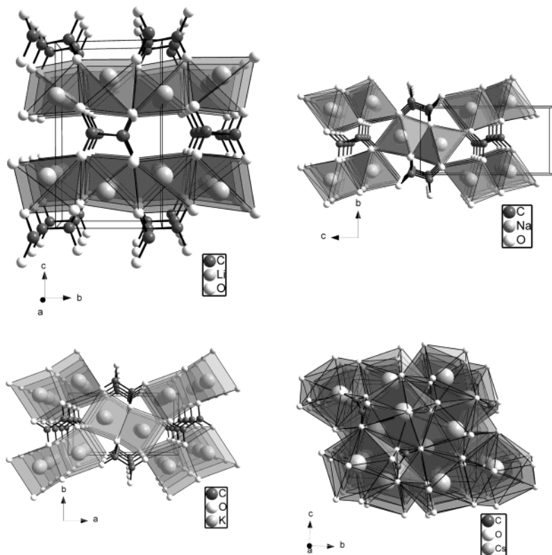
Figure 6. Crystal structures of A_2C_2O_4 [ A = \text{Li} (top left), 16 \text{Na} (top right), 17 \text{K} , \beta - \text{Rb} (bottom left), \alpha - \text{Rb} , \text{Cs} (bottom right)] in different projections. Oxygen positions are in white, carbon positions are in dark gray, and alkali metal positions and their corresponding polyhedra are in light gray.
